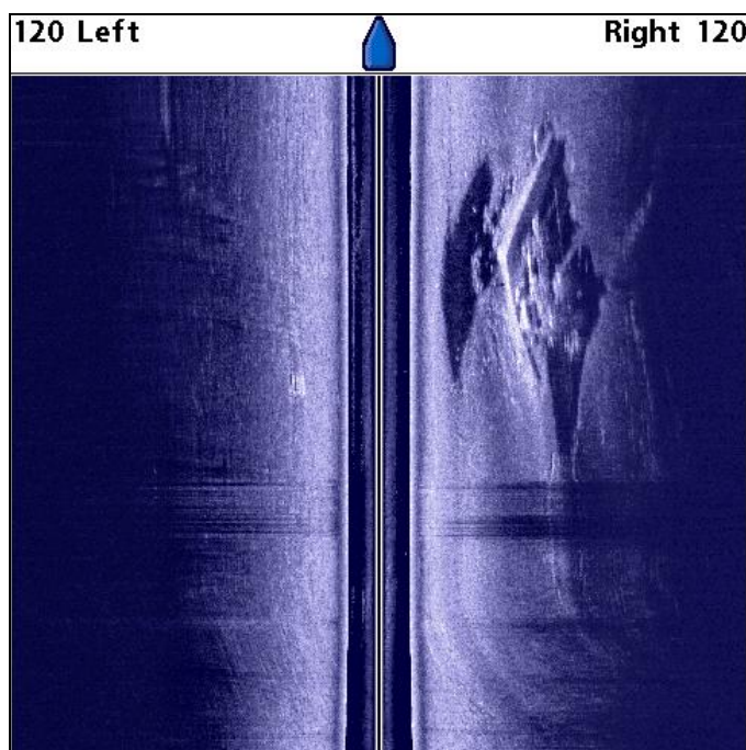
Figure 11. Submerged diamond-shaped ice pier.
