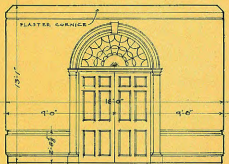
WEST WALL SCALE 1/8" = 1'-0"
